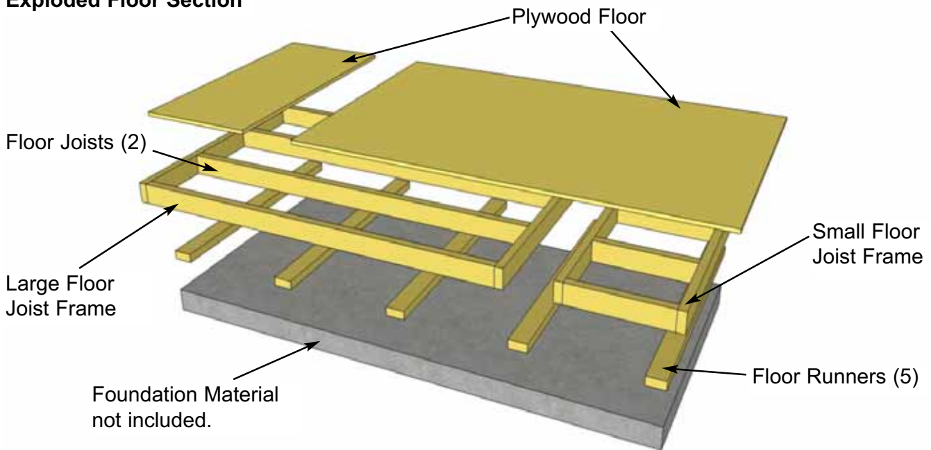
Exploded Floor Section
